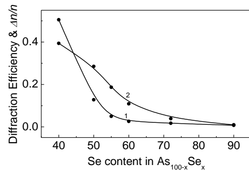
Fig.10. The dependence of the diffraction efficiency (curve 1) and the degree of modification of the refractive index \Delta n/n (curve 2) vs. Se concentration in the As_{100-x}Se_x glassy system.
