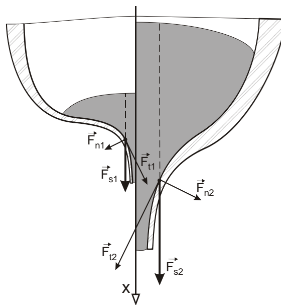
Fig.3. Influence of a melt pressure force on the shape of a primary stretching cone (for the small drop – on the left, for the big drop – on the right).
