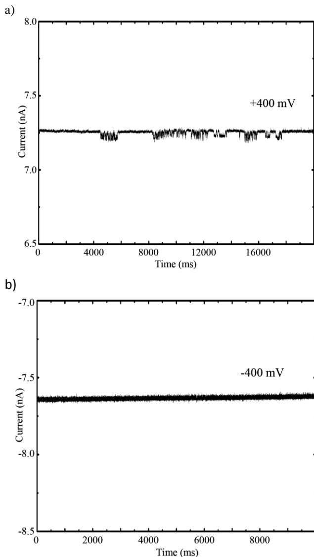
Fig. 4. Particles translocation experiment with pipette of 800 nm pore size, a) shows clear blockade signals with positive +0.4V potential applied, and b) no translocations observed after switching voltage to negative sign.
