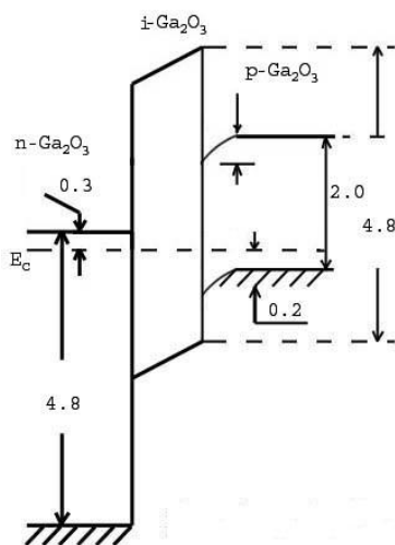
Fig.6. Band diagram of n\text{Ga}_2\text{O}_3-i\text{Ga}_2\text{O}_3-p\text{GaSe: Cd} heterojunction
