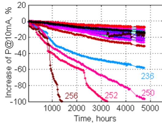
Fig. 9. Plots of changes in power at 10 mA driving current versus time for a set of 24 devices under current and temperature stress
