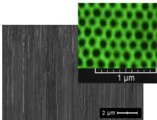
Fig. 3. XRD analyses of the complexes (upper part); hydrogen bonding inside [\text{Ni}(\text{C}_3\text{N}_2(\text{C}_6\text{H}_5)_2\text{NO}_2)_2(\text{CH}_3\text{OH})_2] structure (middle part); SEM image of an InP template filled with coordination compounds. The inset shows a top of view of the pores (lower part).
