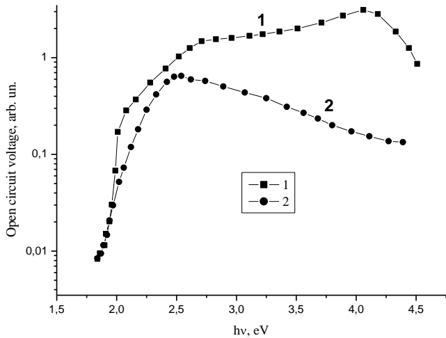
Fig.4. Open circuit voltage spectral distribution of p\text{Ga}_2\text{O}_3/i\text{Ga}_2\text{O}_3-n\text{GaSe} heterojunctions with a layer of native oxide obtained at 480^\circ\text{C} (curve 1) during 90 min and at 700^\circ\text{C} (curve 2) during 90 min in a normal atmosphere. The GaSe lamella thickness is of 11,5\ \mu\text{m}
