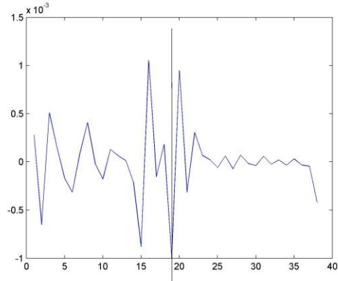
Figure 1: The Scree Test Acceleration Factor
