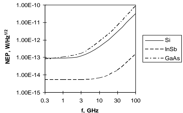
Fig. 5. The calculated noise equivalent power dependence on the signal frequency for contacts HTSC-semiconductor. The legend inscriptions and other data are similar to those in fig. 4. T = 77.4 K.
