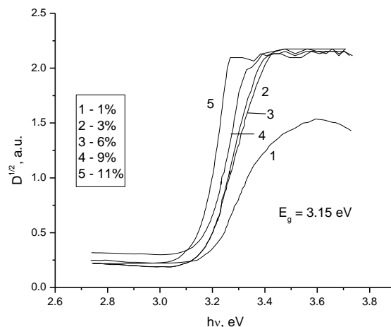
Fig.4. The optical density transmission spectra of samples of thin layers of NC on glass substrates for different concentration of Eu(TTA)_2(Ph_3PO)_2NO_3 in PVP at room temperature ( T=293 K).
