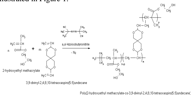
Fig. 1. Idealized copolymerization process
