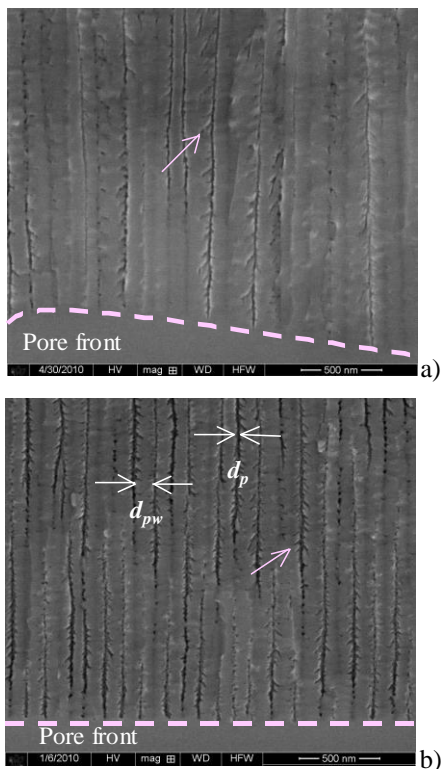
Fig. 2. SEM pictures of a cross section for pores in nucleation stage electrochemically etched a) 15 s, 2V; b) 30 min, 2V into n-type Si for (0.02–0.05) Ω·cm resistivity.
