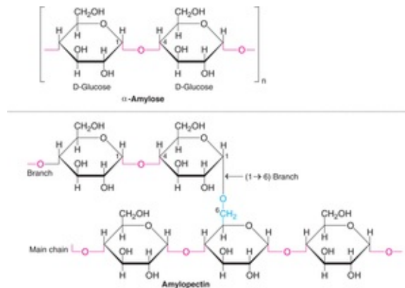
FIG. 2.13 Structure of starch ( \alpha -amylose and amylopectin).
