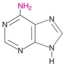
Adenine (A) (6-aminopurine)
