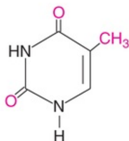
Thymine (T) (2,4-dioxy-5 methylpyrimidine)
