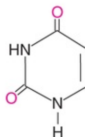
Uracil (U) (2,4-dioxypyrimidine)
