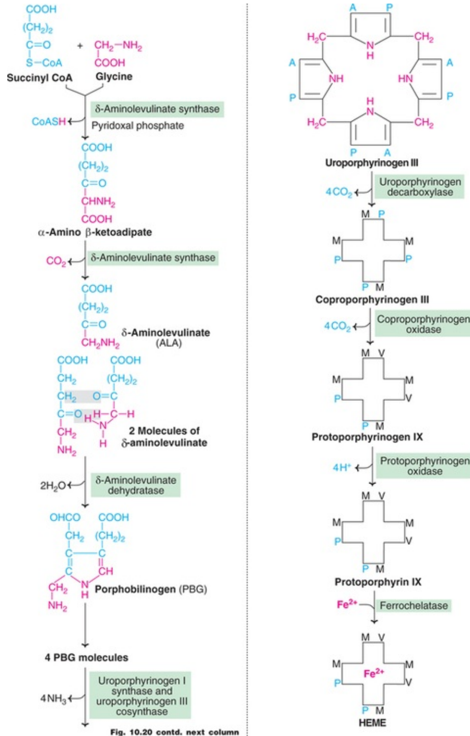
FIG. 10.20 Biosynthesis of heme [A–Acetyl ( -\text{CH}_2\text{-COO}^- ); P–Propionyl ( -\text{CH}_2\text{-CH}_2\text{-COO}^- ); M–Methyl ( -\text{CH}_3 ); V–Vinyl ( -\text{CH}=\text{CH}_2 )].
