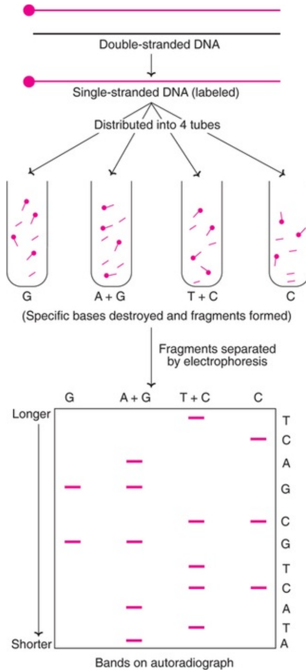
FIG. 27.10 Maxam and Gilbert method for DNA sequencing.
