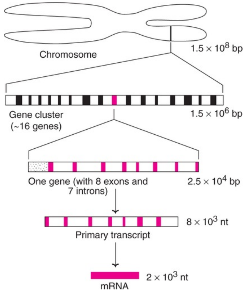
FIG. 25.11 A diagrammatic representation of the relationship between eukaryotic chromosomal DNA and mRNA (bp–Base pair; nt–Nucleotides).
