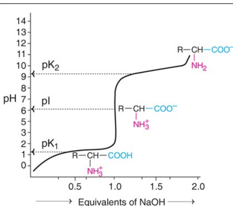
FIG. 4.3 Titration curve of an amino acid-leucine ( R = (\text{CH}_3)_2\text{—CH—CH}_2 —; pK_1 = Dissociation constant for COOH; pI = Isoelectric pH; pK_2 = Dissociation constant for \text{NH}_3^+ ).
