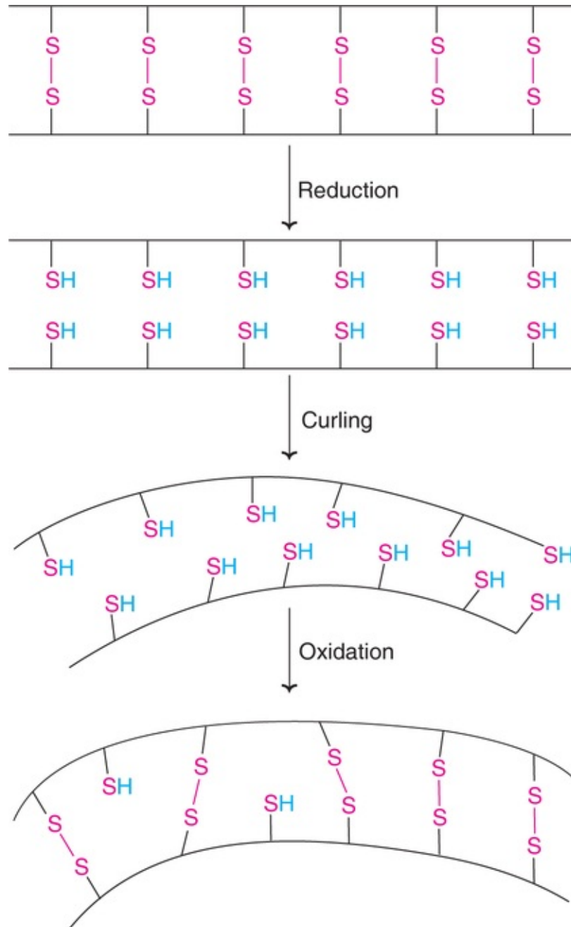
FIG. 22.2 A diagrammatic representation of hair waving with suitable alterations in keratin structure (-S-S corresponds to disulfide bonds of cysteine; -SH indicates sulfhydryl groups of cysteine)
