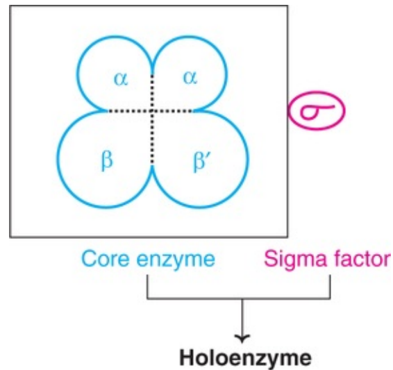
FIG. 25.2 RNA polymerase of E. coli .
