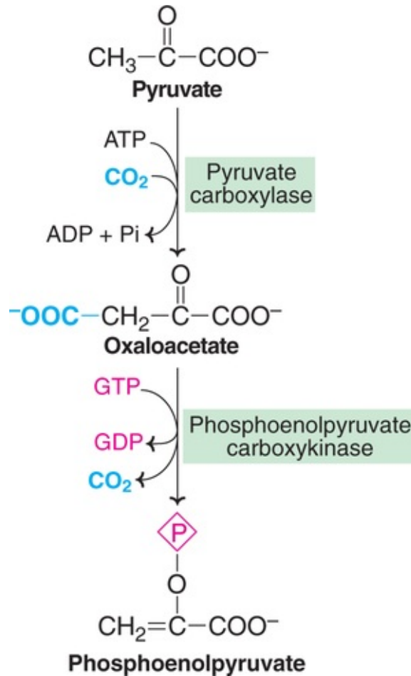
FIG. 13.12 Conversion of pyruvate to phosphoenolpyruvate.
