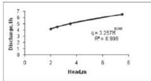
Fig. 2.4 Head discharge relationship for the drippers of 5 l/h nominal discharge
