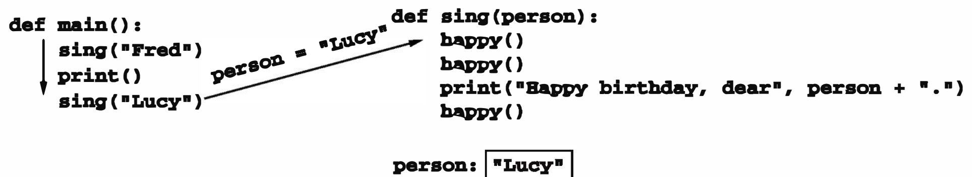
Figure 6.4: Snapshot of second call to sing
