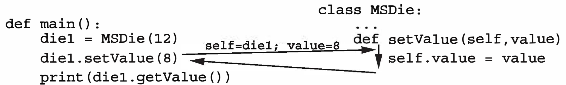
Figure 10.2: Flow of control in call: die1.setValue(8)
