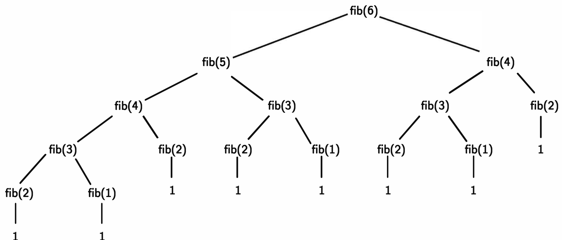
Figure 13.2: Computations performed for fib(6)
