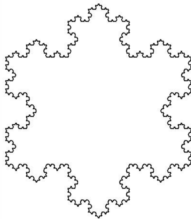
Figure 13.7: Koch snowflake
