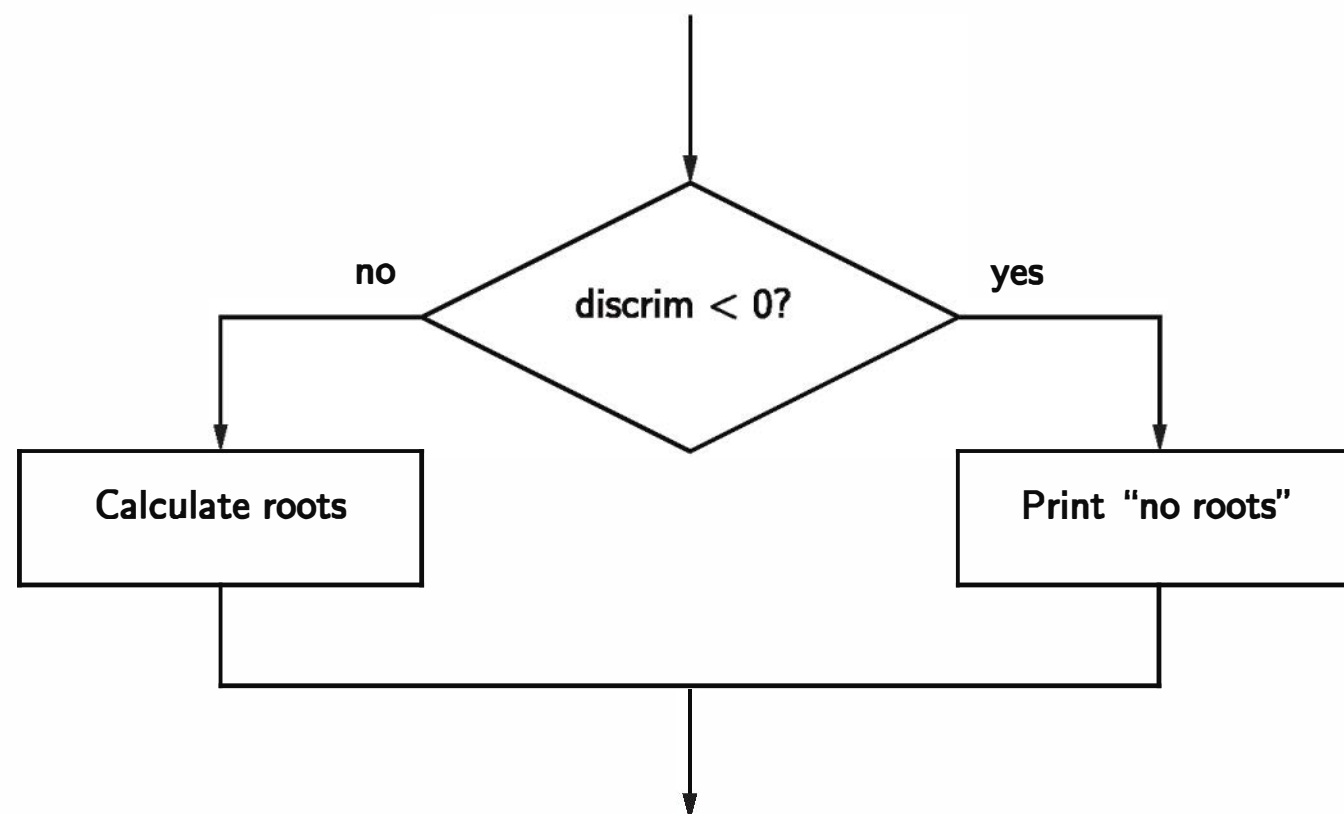
Figure 7.3: Quadratic solver as a two-way decision
