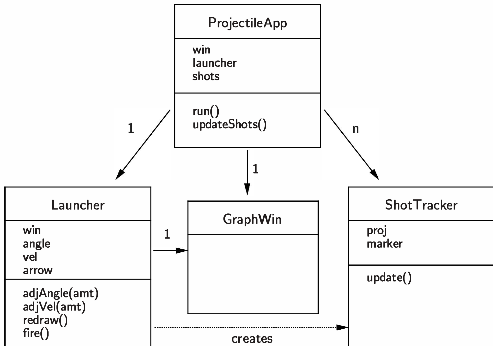
Figure 11.3: Class diagram for the multi-shot animation
