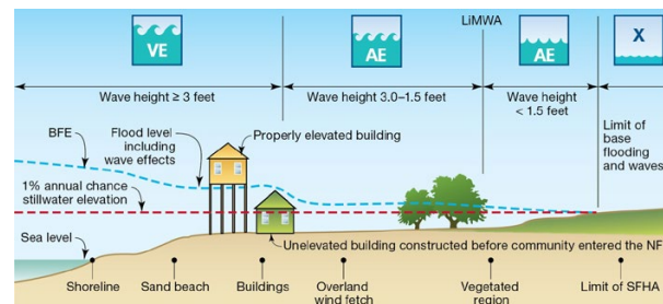
Typical Shoreline Perpendicular Transect Showing Stillwater and Wave Crest Elevations and Associated Flood Zones. (Adapted after Figure 3-53, FEMA, Coastal Construction Manual: Principles and Practices of Planning, Siting, Designing, Constructing, and Maintaining Residential Buildings in Coastal Areas (Fourth Edition) FEMA P-55, Volume I, August 2011.)
